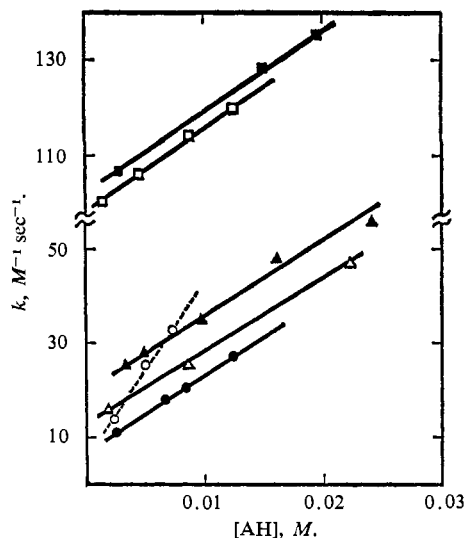
Figure 1. Plots of second-order rate constant, k , vs. [acid] for the reaction of p -benzoquinone with sodium thiosulfate at 19.5 \pm 0.3^\circ : HCl-KCl buffer: \blacksquare , pH 1.2; \square , pH 1.6; AcOH-AcONa buffer: \blacktriangle , pH 3.2; \triangle , pH 3.8; \bullet , pH 4.7; -\text{O}- , pH 4.7 in 20% EtOH.
